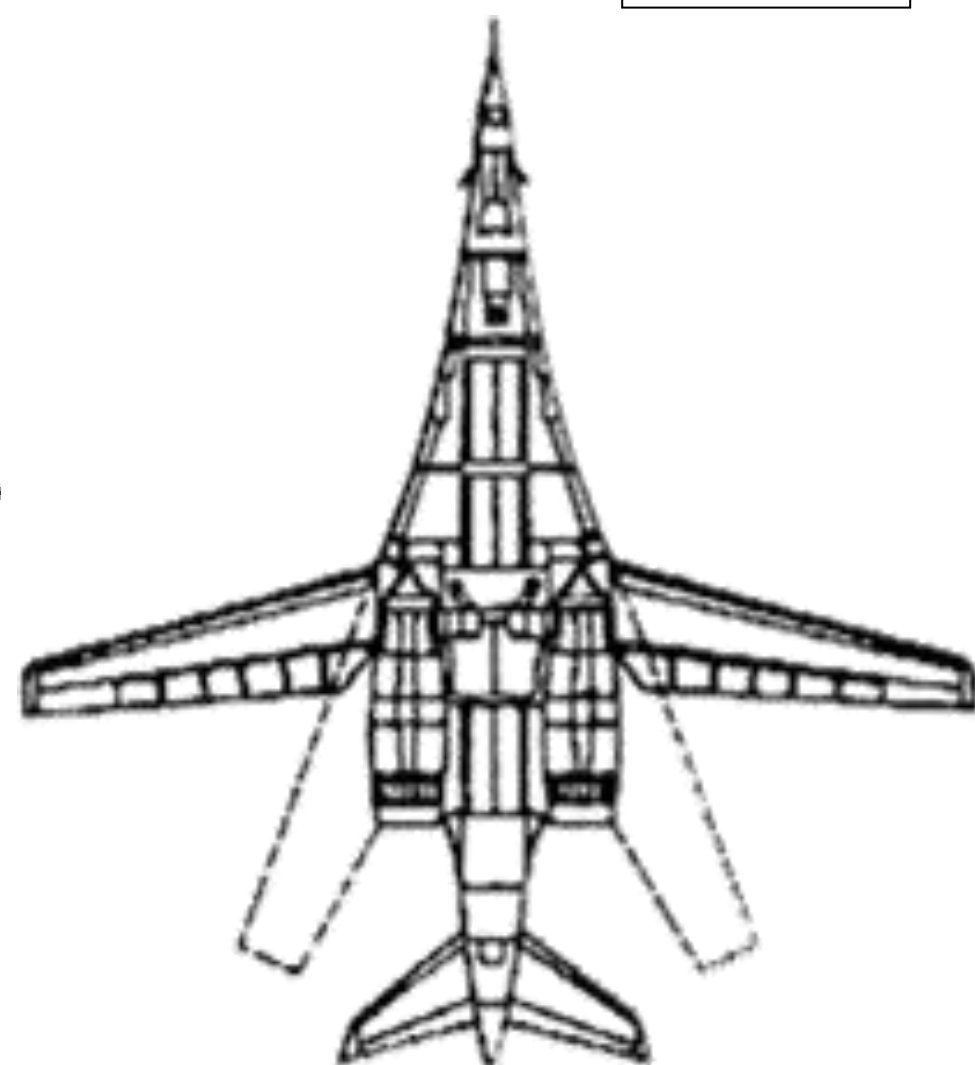
B-1B Lancer W: Extended 41.8m W: Swept Aft 24.1m L: 44.5m
